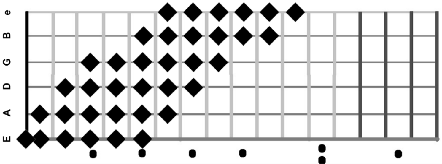
Fig. 1: Guitar Tab of the Chromatic Scale
